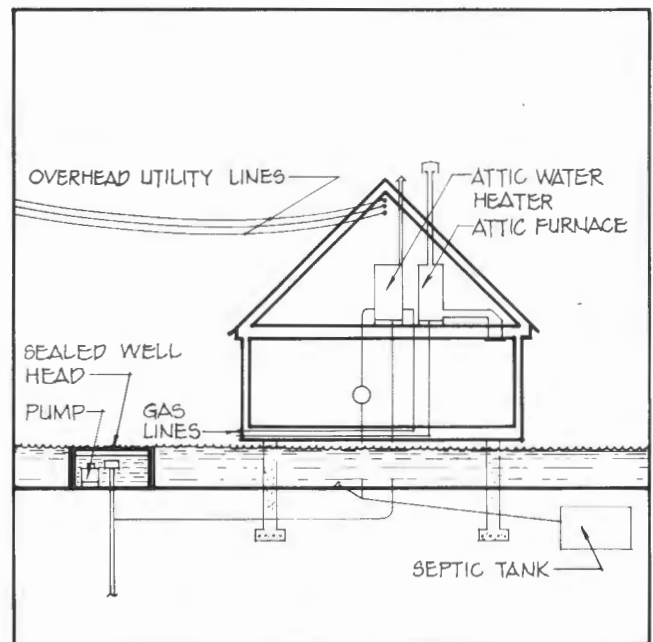
Figure 4.50. Locating Utilities
